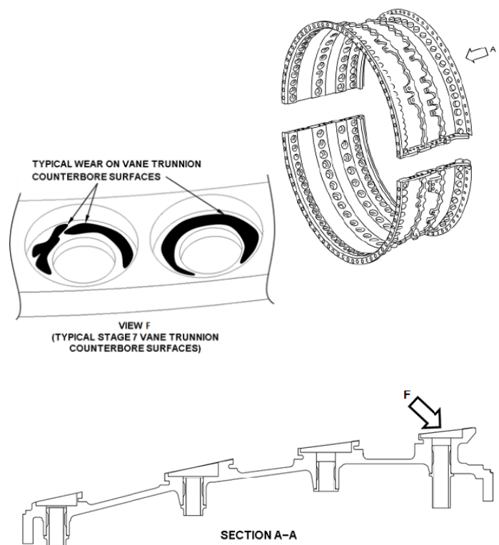
Figure 1: PW4000 112" HPC Front Case - 7th Stage Trunnion Counterbores
