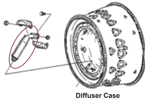
Figure 1: Location of No. 4 Bearing Scavenge Oil Tube Assembly
